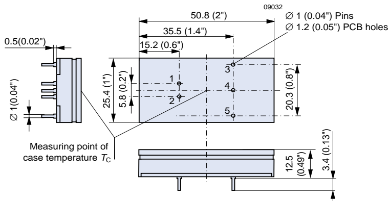
Fig. 22 Case IMX 7 with C pinout (option C) for double output units, pins 6 and 7 are not fitted. With single output units pins 4, 6 and 7 are not fitted. Weight: <24 g
