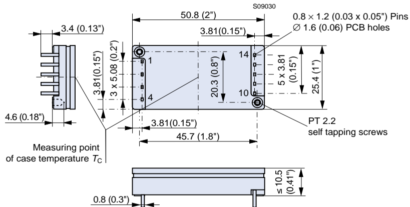
Fig. 21 Case IMX 7 with standard soldering pins Weight: <20 g
