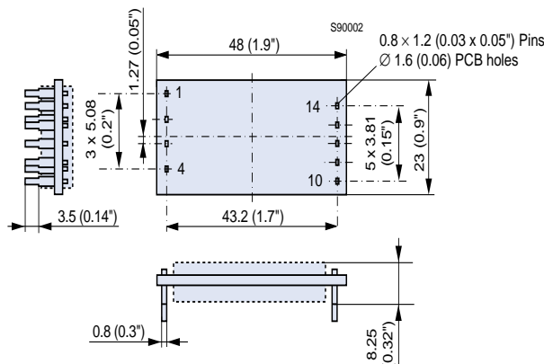
Fig. 22 Case IMX 7 with C pinout (option C) for double output units, pins 6 and 7 are not fitted. With single output units pins 4, 6 and 7 are not fitted. Weight: <24 g
