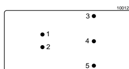
Fig. 25 Pin allocation C pinout, bottom view
