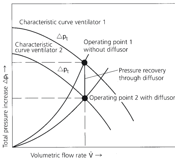
Figure 2: Pressure recovery
