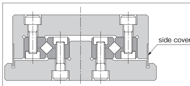
Figure 7. Example of Dust Prevention Mechanism
