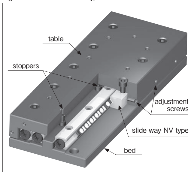
Figure 2. Structure of NVT type
