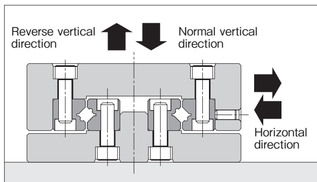
Figure 6. Direction of Load
