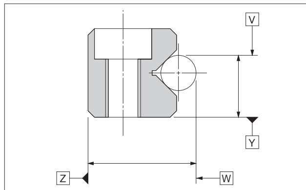
Figure 5. NVT type Accuracy Measurement
