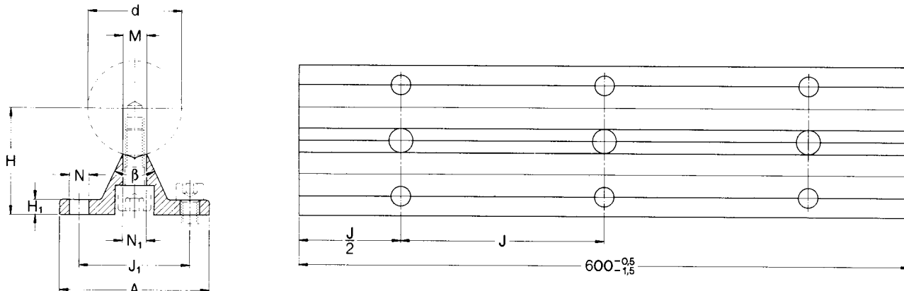
Shaft support with bore holes LRCB design
