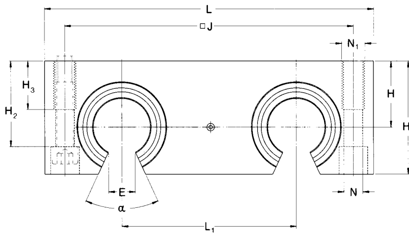
LQCF..2LS design
