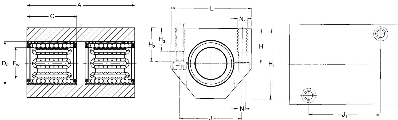
LTBR linear bearing unit with integral double lip seals
