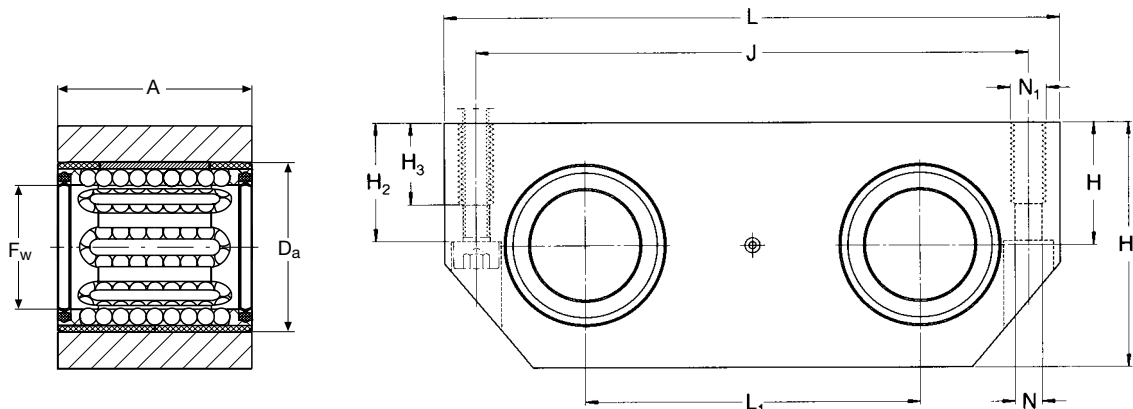
LDTR linear bearing unit with integral double lip seals
