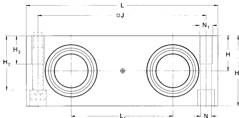
LQCD..2LS design
