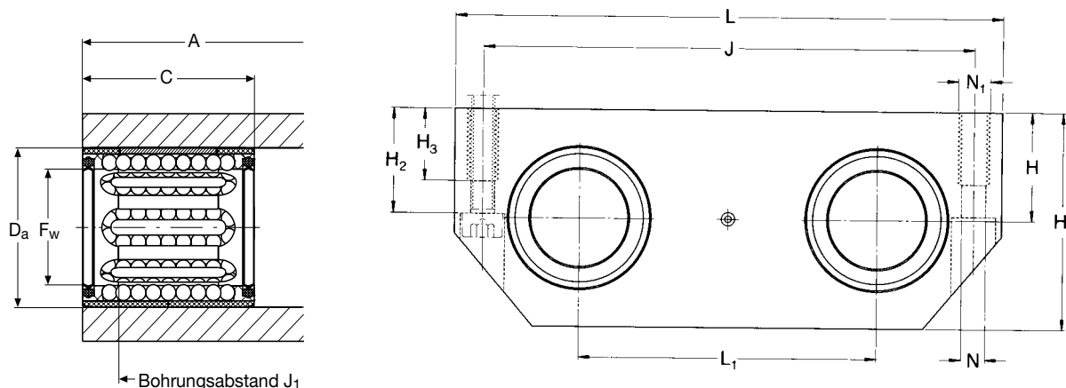
LQBR linear bearing unit with integral double lip seals
