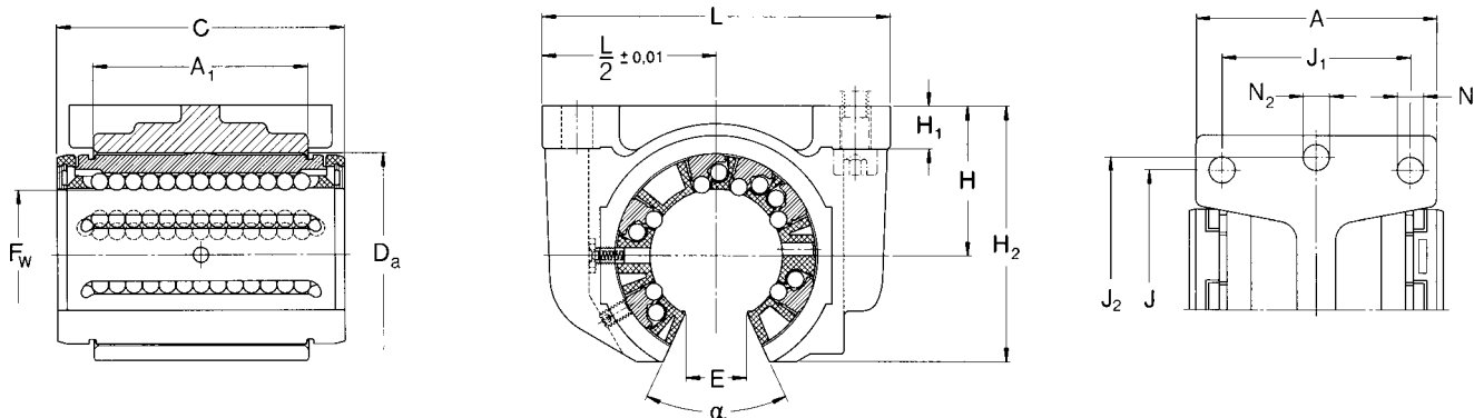
Linear bearing unit with 2 shields
