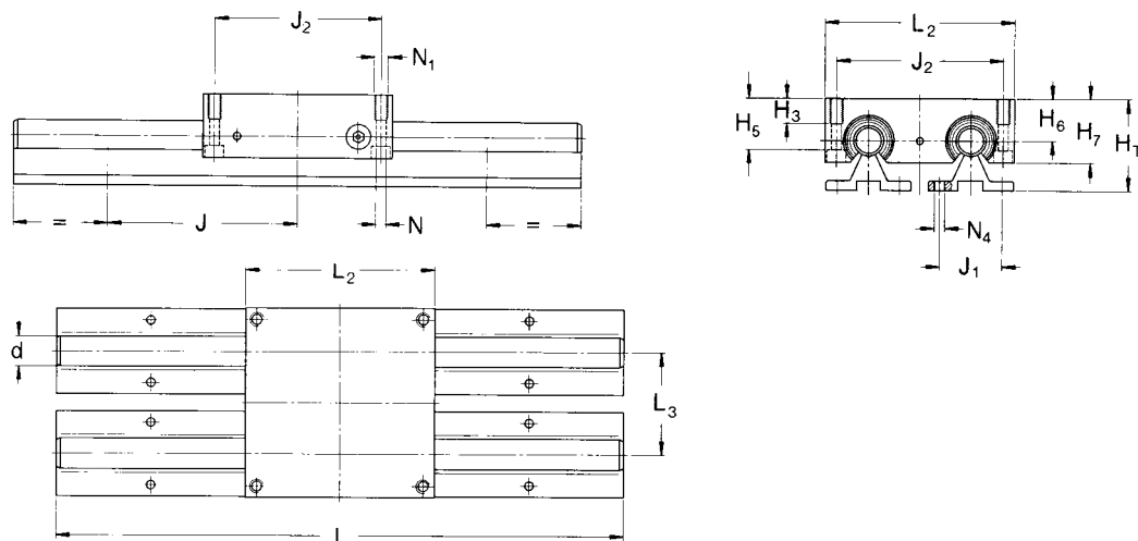
Design LZAU with open linear bearing unit
